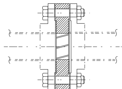
▶ Perturbateur type "Tourbillon"
